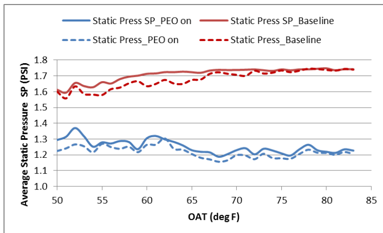
Figure 3. Example of comparison of control setpoints during the baseline and optimizer (post-installation) periods
