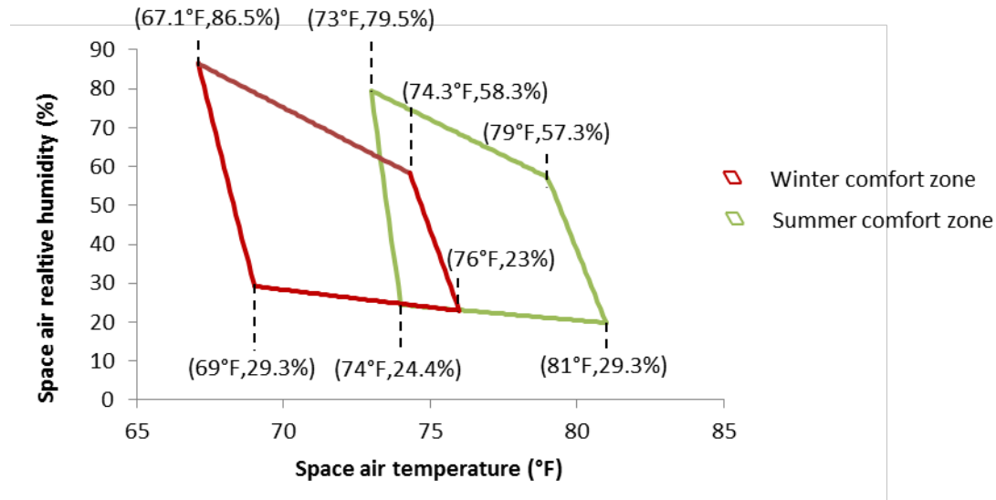
Figure 2. A simplified representation of the ASHRAE thermal comfort model, with comfort as a function of relative humidity and air temperature
